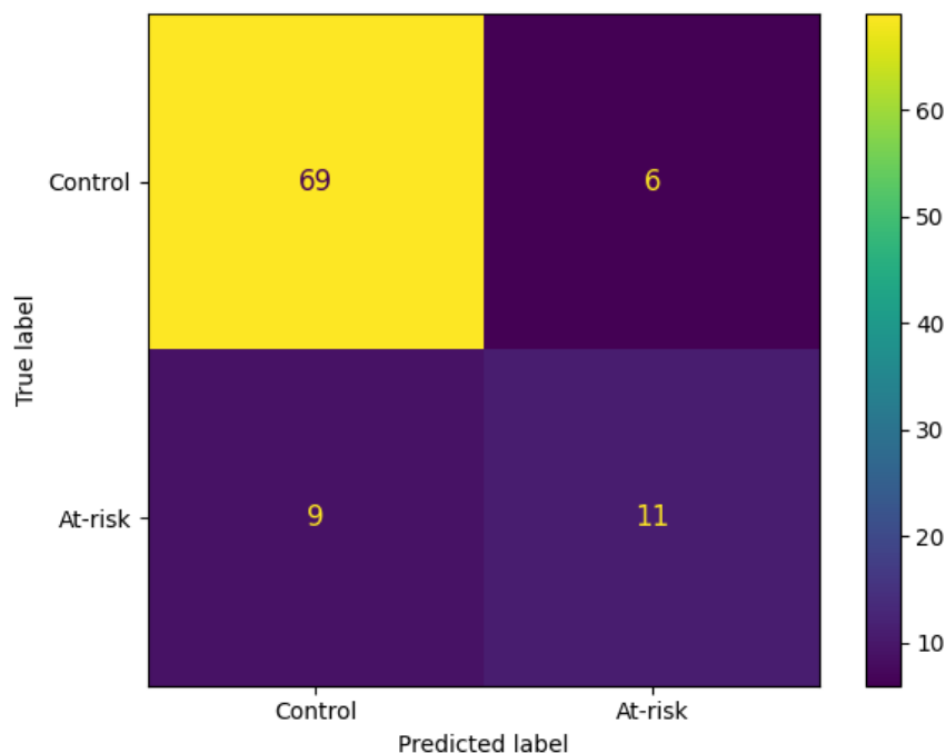
Fig 1: Confusion matrix
